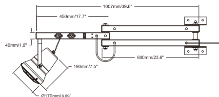
Double Arm with the 2 of receptacles
