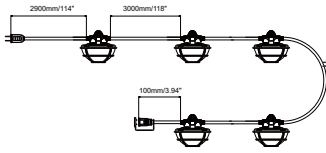
Option 1: It has 5 LED light heads and comes with a 50ft/ AC cord. Light heads spaced 10 feet/3mts apart
